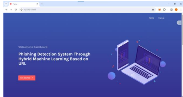
Fig 18 Home page
