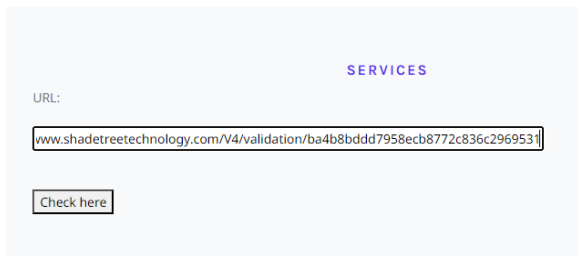
Fig 21 User input
