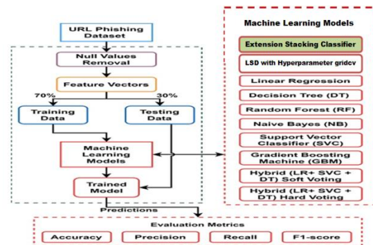
Fig 1 Proposed architecture
