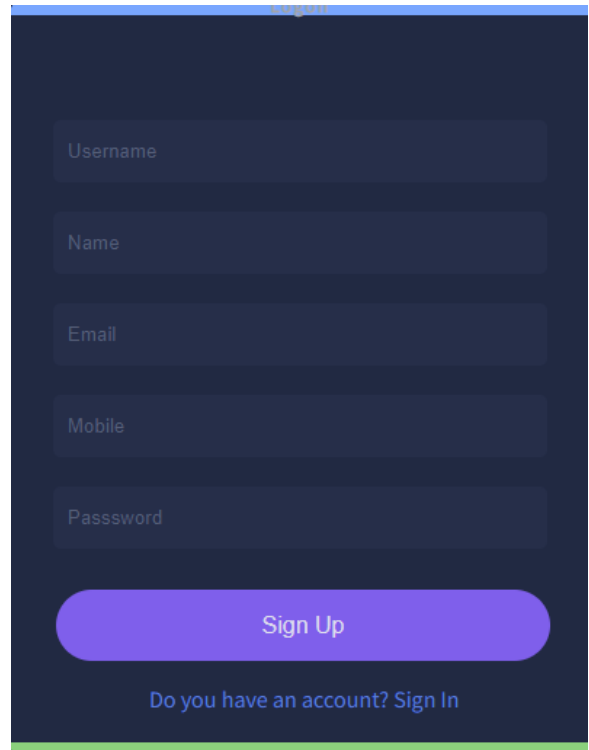
Fig 19 Signin page
